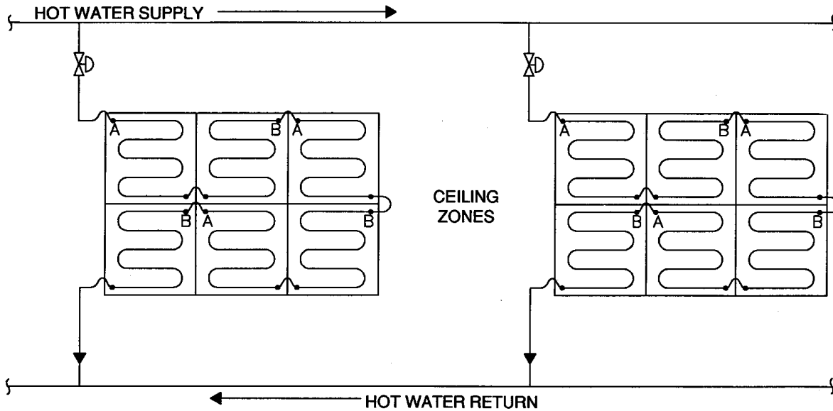
TWO-PIPE SYSTEM
